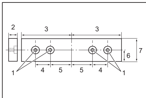
► 1. Hole 2. Over 15 mm (9/16") 3. Over 270 mm (10-5/8") 4. 90 mm (3-1/2") 5. 145 mm (5-3/4") 6. 19 mm (3/4") 7. 115 - 120 mm (4-1/2" - 4-3/4")
